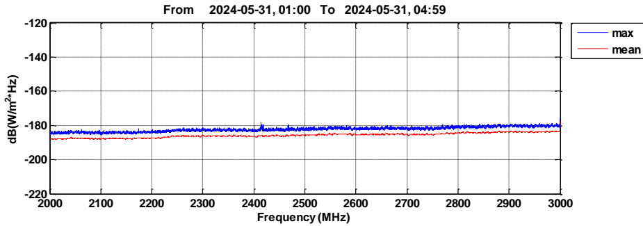
Fig.6 RFI scan of 2000-3000MHz in nighttime.
