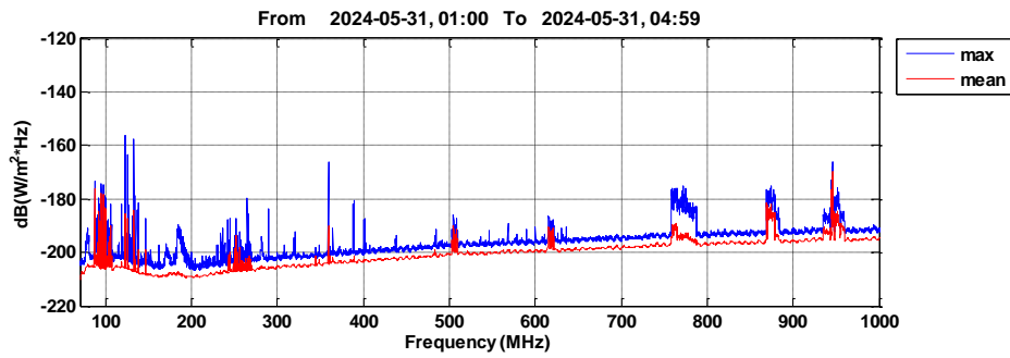
Fig.2 RFI scan of 70-1000MHz in night time.
