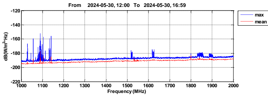
Fig.3 RFI scan of 1000-2000MHz in daytime.
