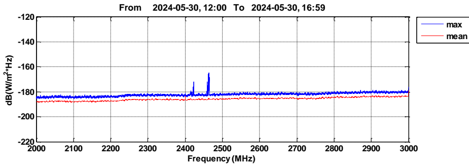
Fig.5 RFI scan of 2000-3000MHz in daytime.
