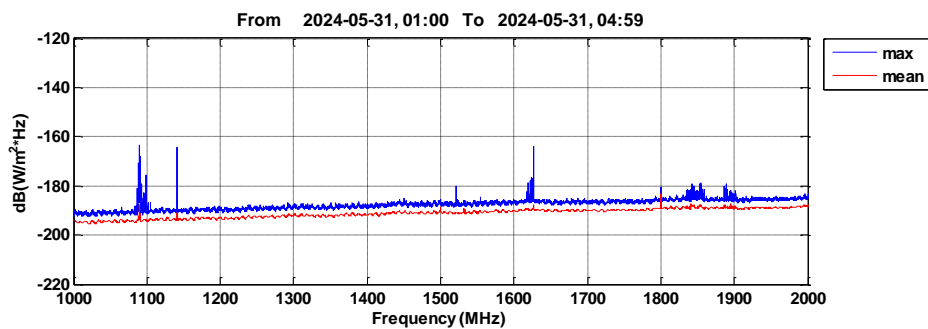
Fig.4 RFI scan of 1000-2000MHz in nighttime.
