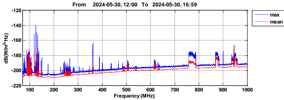
Fig.1 RFI scan of 70-1000MHz in daytime.
